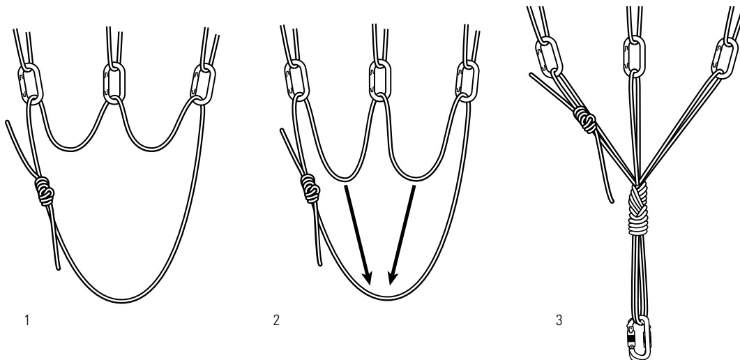
PRE-EQUALIZATION WITH CORDELETTE
