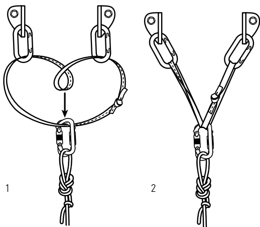
TWO-POINT SELF-EQUALIZATION
