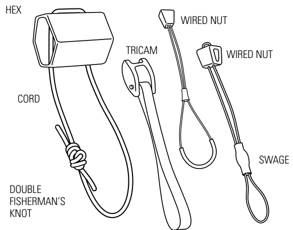
Chocks are available in a wide variety of shapes and sizes.
