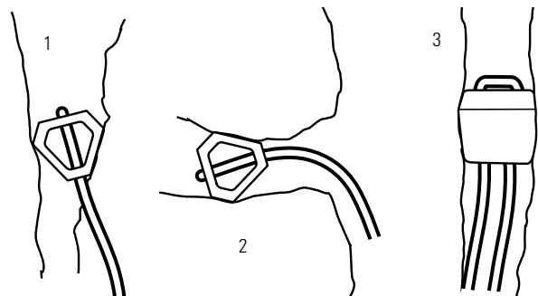
1) In a vertical crack, as a passive cam—good contact with the rock gives greater holding power. 2) In a horizontal crack, as a passive cam—the sling exits near the roof of the crack for proper camming action. 3) Sideways in a crack, as a passive cam.
