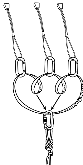
THREE-POINT SELF-EQUALIZATION
